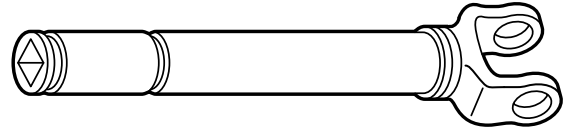
Yoke, Tube & Slip Sleeve Assy. – Part No. 1449 Ear Hole Centerline to End 33-5/8"
