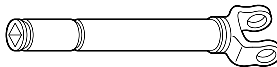
Yoke, Tube & Slip Sleeve Assy. – Part No. 1349 Ear Hole Centerline to End 36-1/8"
