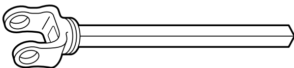
Yoke & Shaft Assembly – Part No. 1347 Ear Hole Centerline to End 35-5/8"
