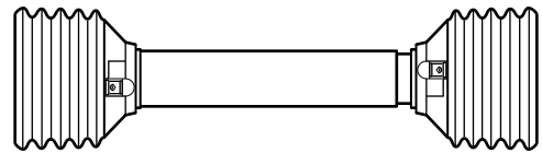
Plastic Safety Shield – Part No. 2072 (Bearing Kit not included) Bearing Kit – Part No. 2086
