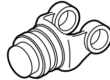
Weld Yoke – Part No. 1475 For 2-3/4" – .109" Wall Tube
