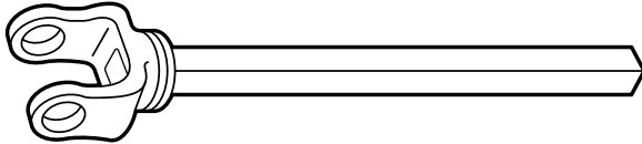
Yoke & Shaft Assembly – Part No. 1447 Ear Hole Centerline to End 33-1/8"
